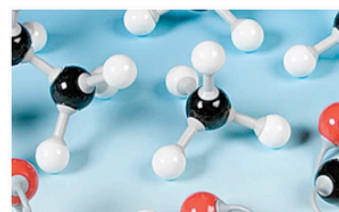
Build Models of Molecules
