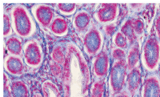
Make Your Own Cell Kit
