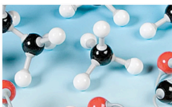
Identifying Chemical Reactions
