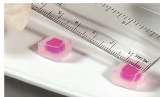
Diffusion and Osmosis Kit
